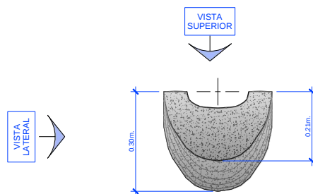
VISTA FRONTAL Escala 1 / 12.5
